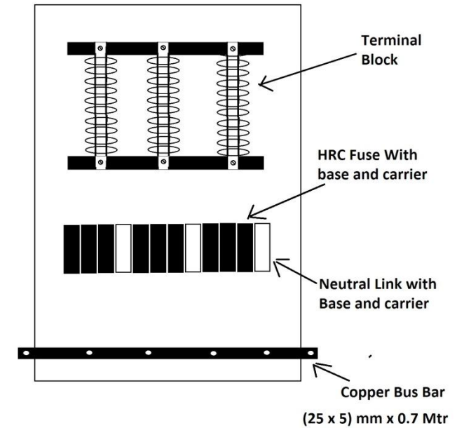
132 & 33 KV CVT/PT Console Box i) TB (CATD-M4) : 30Nos (10x3) ii) 20 A, 550 VAC Fuse Base with Carrier : 9 Nos iii) 20A,550VAC Neutral Link Base with Carrier : 3 Nos
