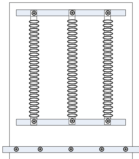
132 KV CT Console Box TB: 72 Nos.(24×3)
