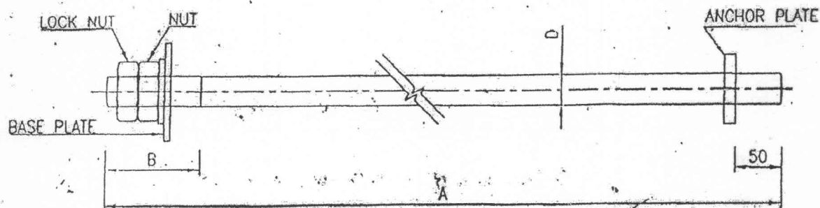
FOUNDATION BOLT
