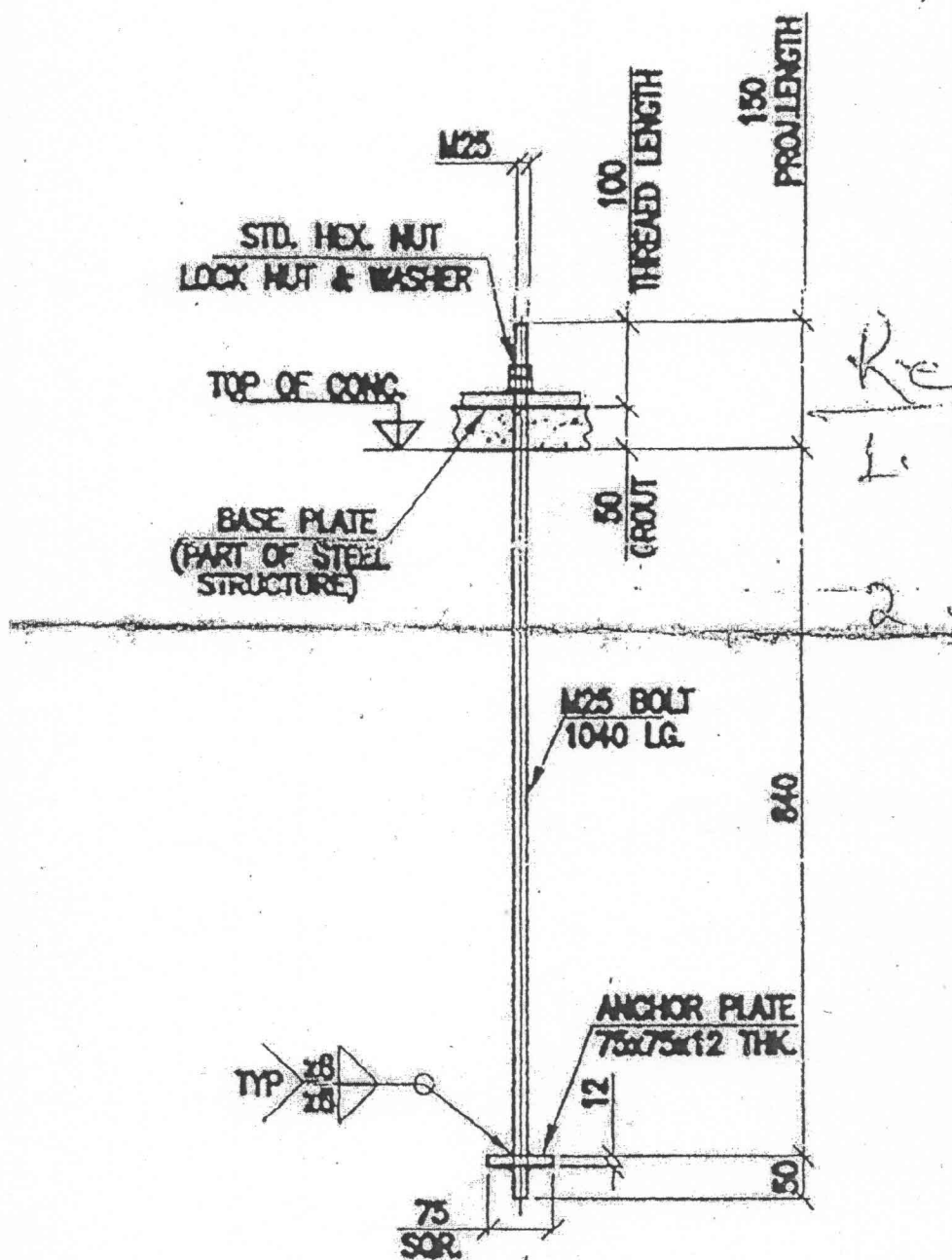
TYP. DETAIL OF FDN BOLT M25x1040mm (SC. 1:10)
