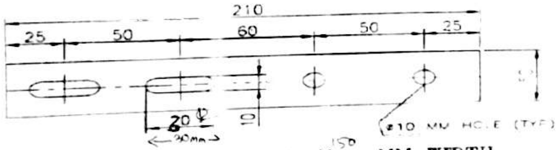
COUPLER PLATE FOR 300/250 MM WIDTH
