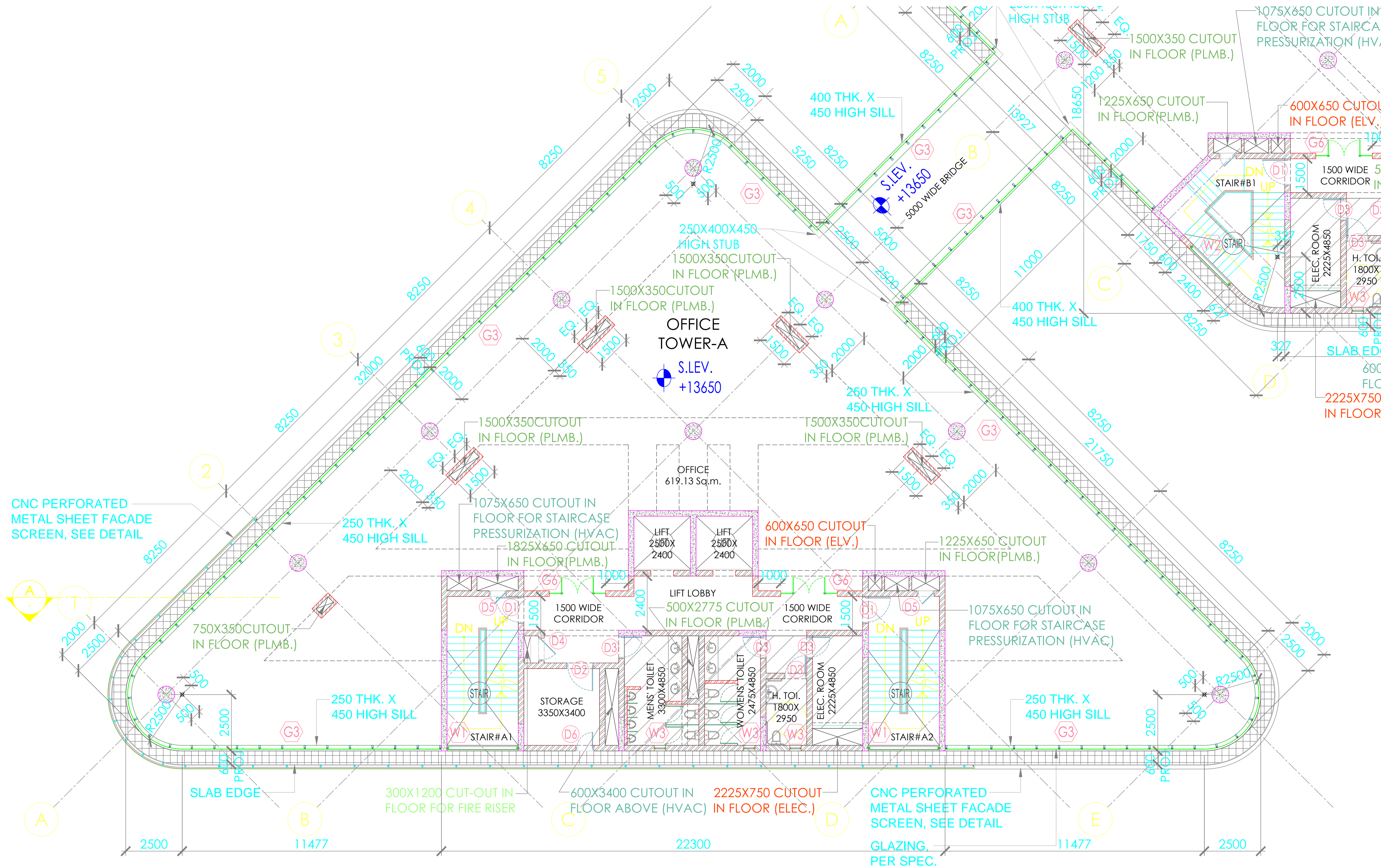
1 THIRD FLOOR LAYOUT PLAN SCALE 1:200
