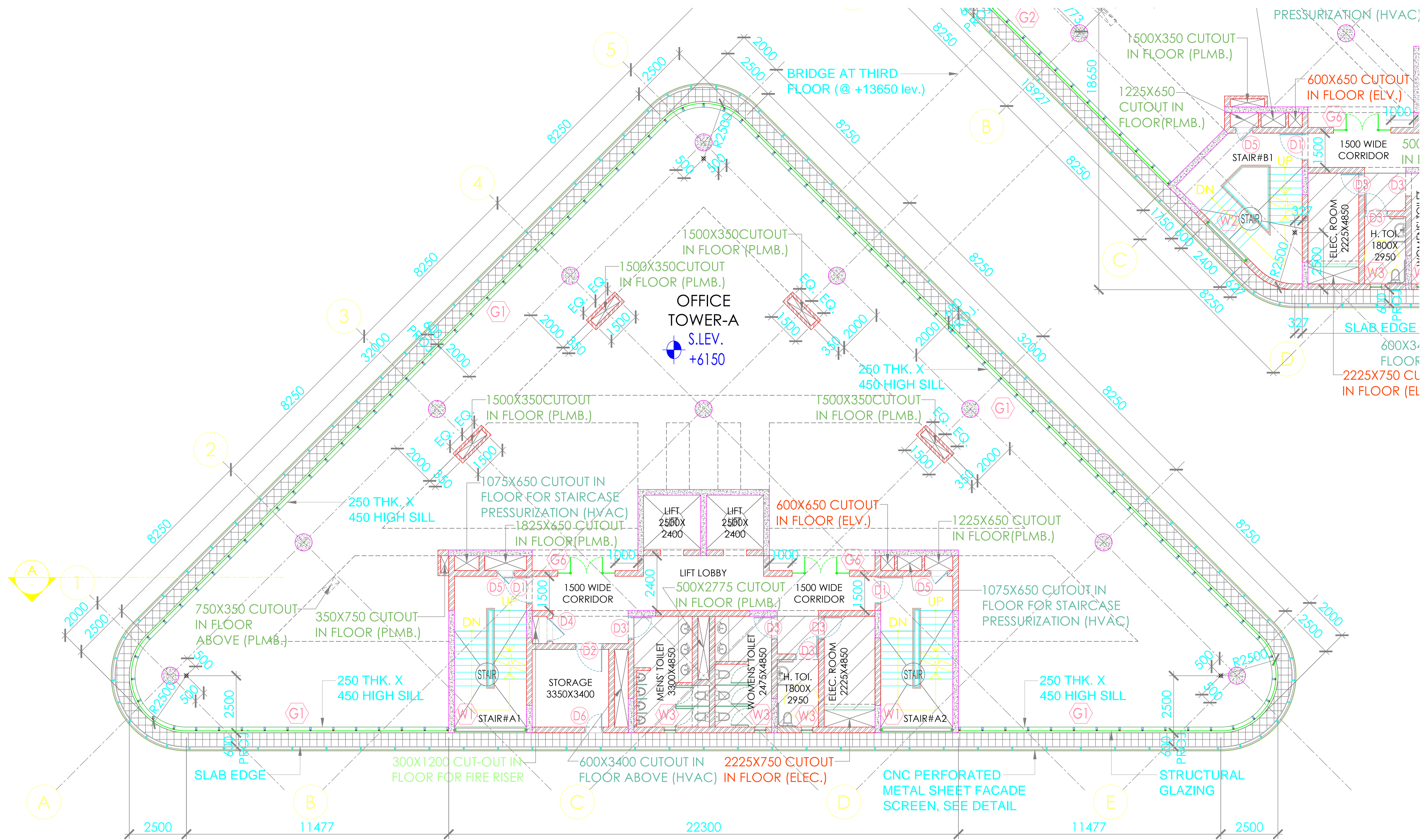
1 FIRST FLOOR LAYOUT PLAN SCALE 1:200
