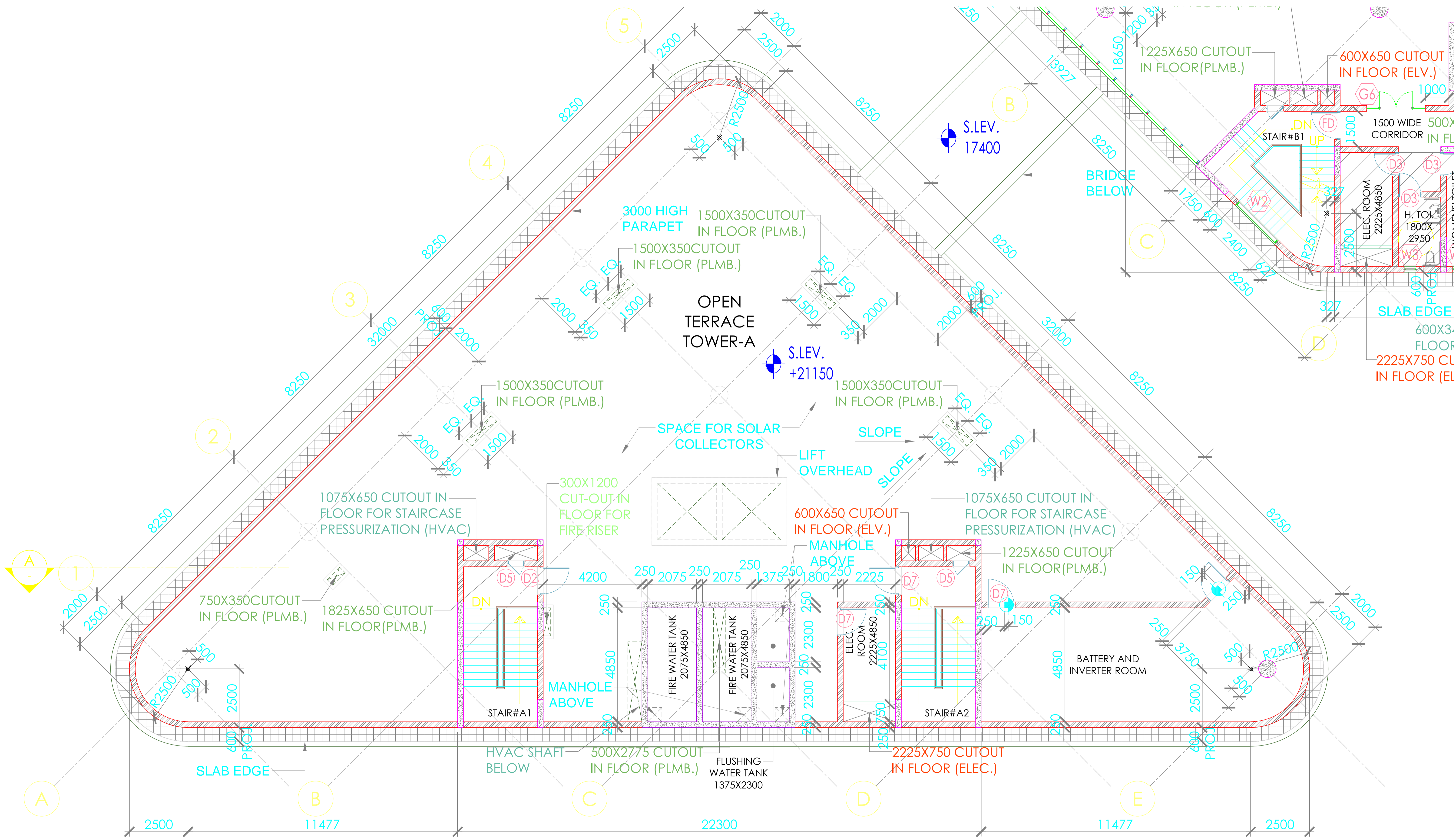
2 FIFTH FLOOR LAYOUT PLAN SCALE 1:200
